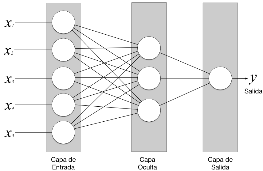
Figura 54: Red neuronal artificial multicapa
