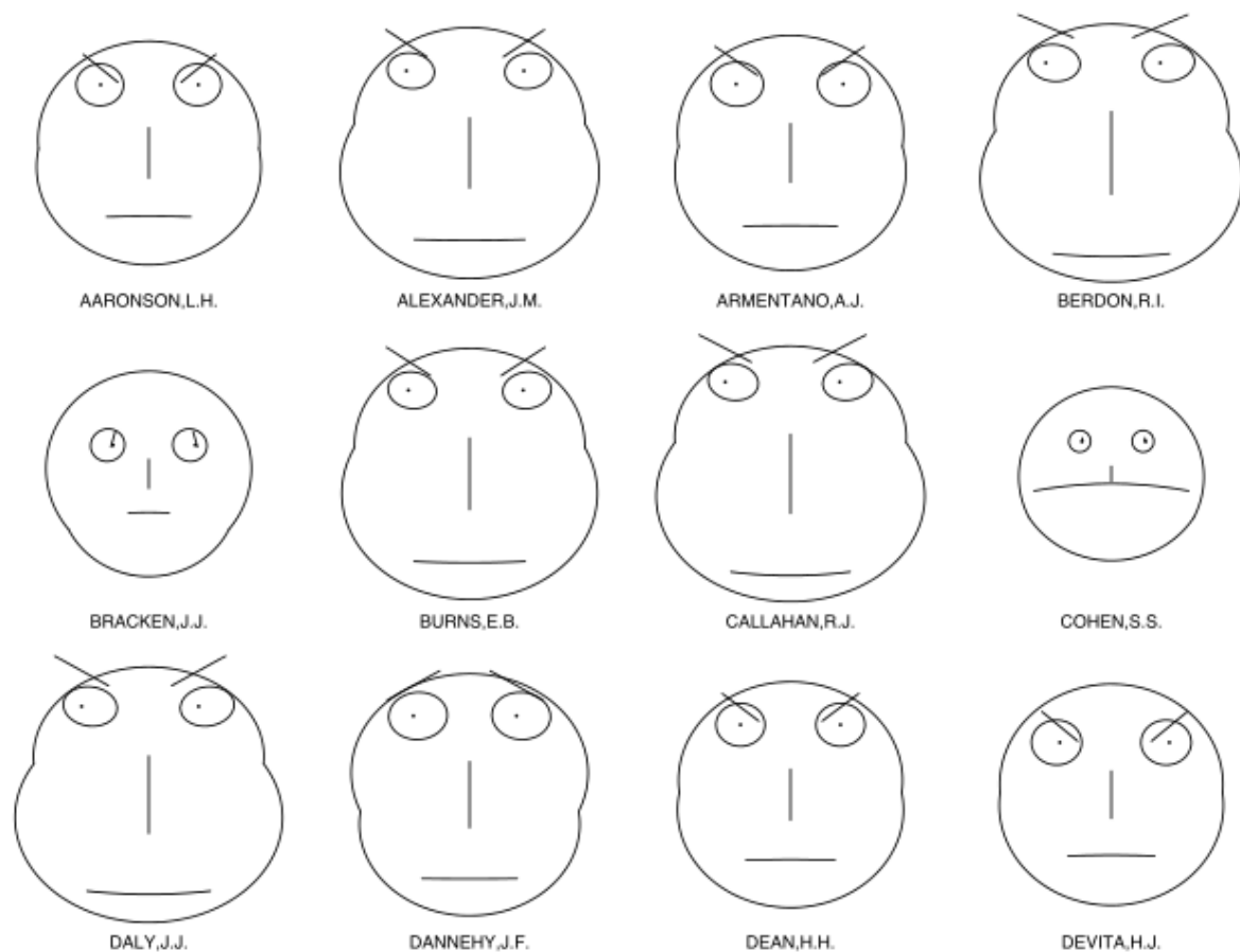
Figura 37: Chernoff_faces
