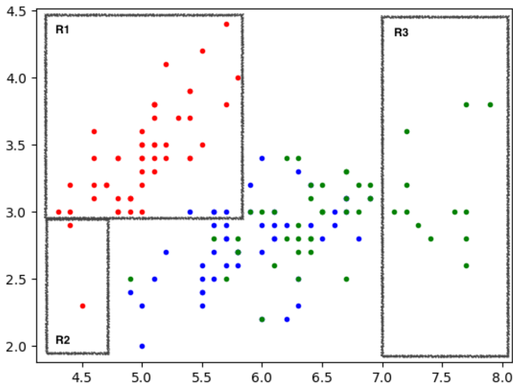
Figura 8: Setosa, Virginica, Versicolor
