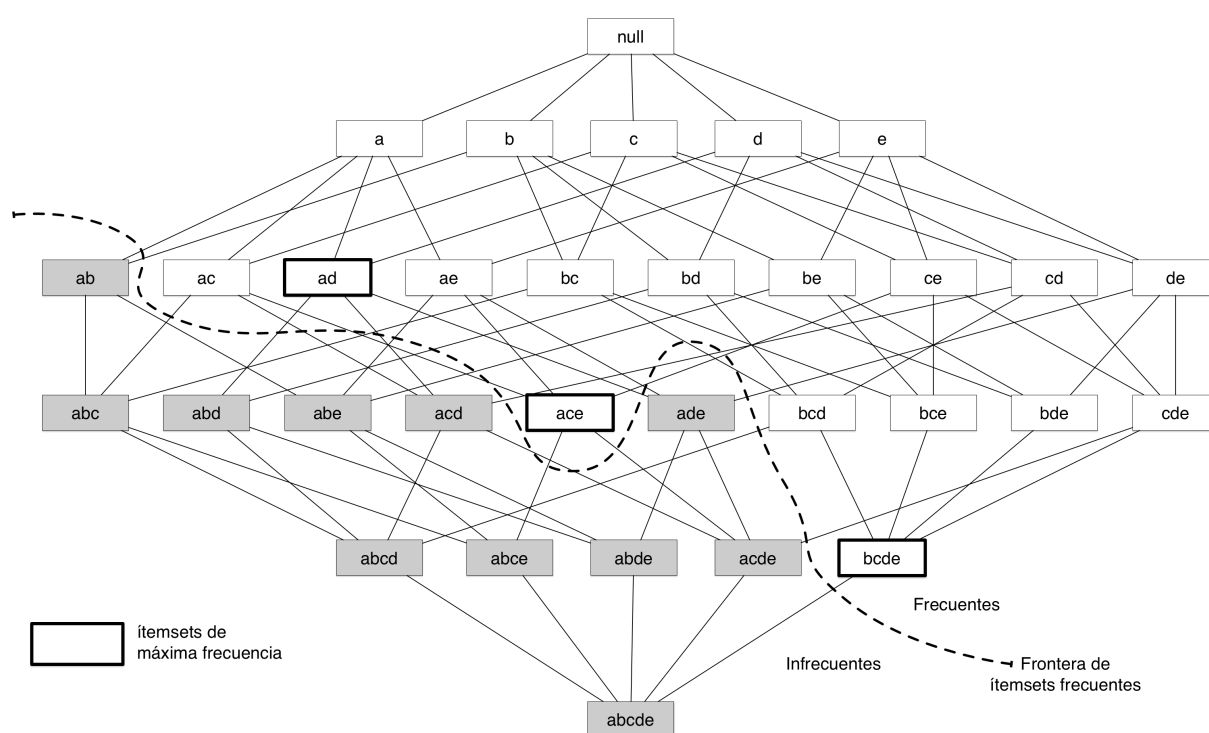
Figura 61: Rejilla de ítemset Tan, Steinbach, and Kumar (2007)
