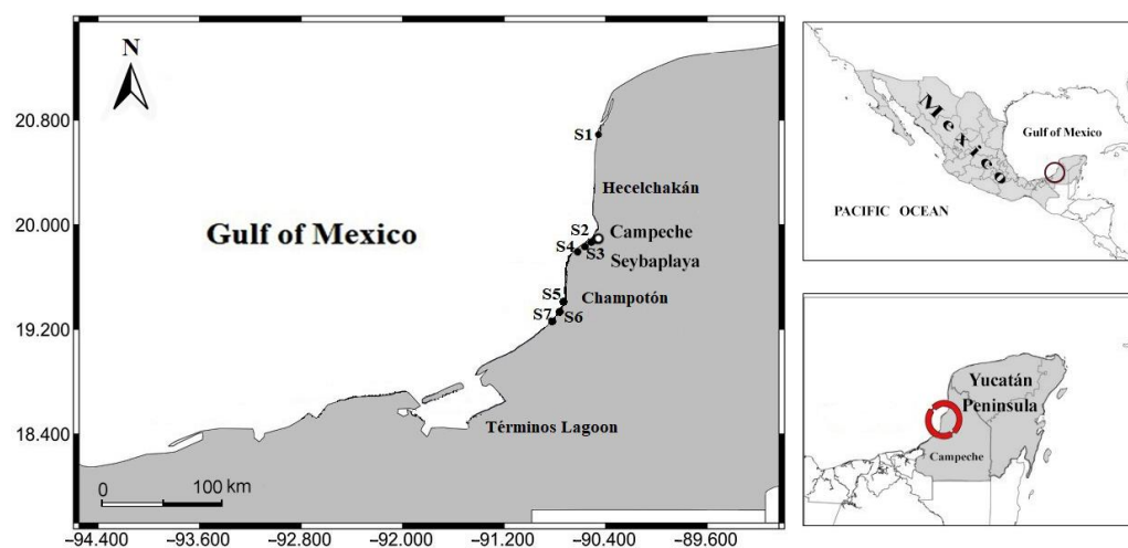
Figure 1. Sampling sites (S1–S7; marked by black circles) in the coastal waters of the State of Campeche. On the maps to the right, red circles indicate the study area.
